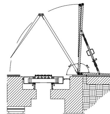
Opening and closing of the MAURER Modular Bridging System
