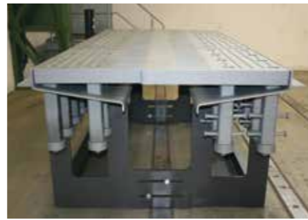
Neglectable maintenance – controlled prestress
