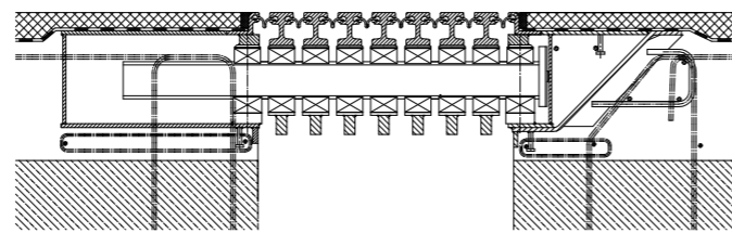
MAURER Fuse Box
